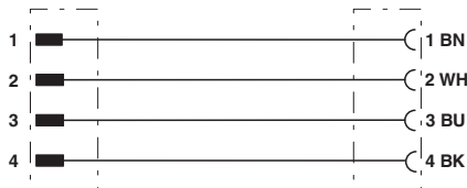
Contact assignment of 7/8" plugs/sockets
